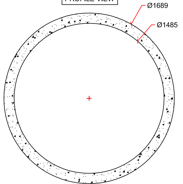
PROFILE VIEW
