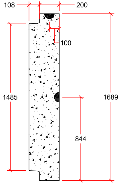
PROFILE VIEW
