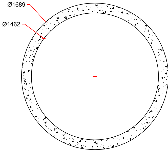
PROFILE VIEW
