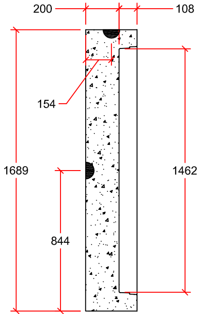
PROFILE VIEW
