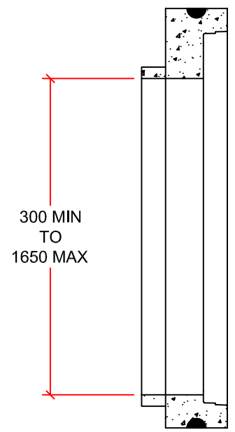
DECREASER
