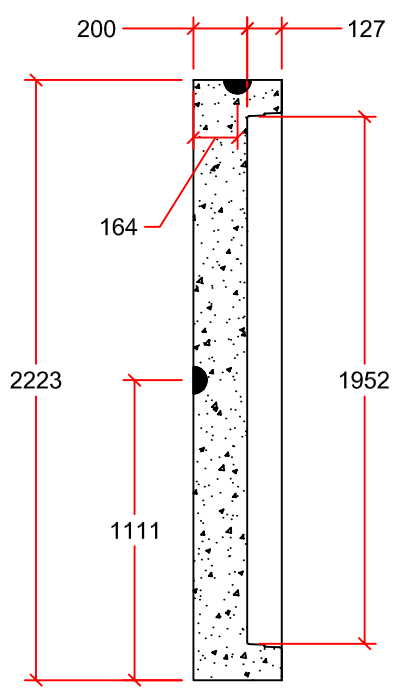
PROFILE VIEW
