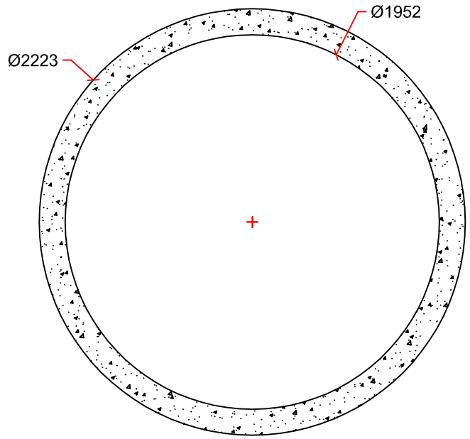
SECTION DETAIL
