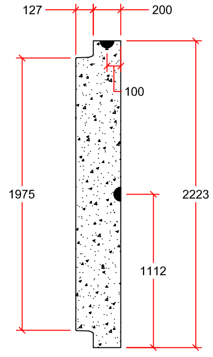
PROFILE VIEW
