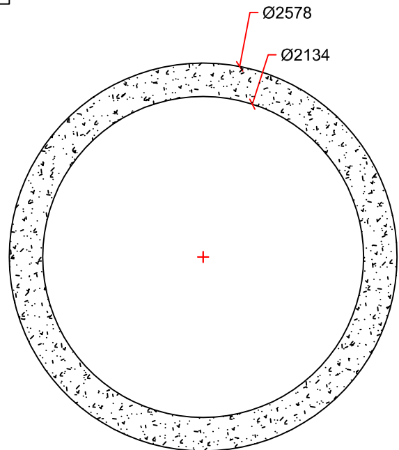
SECTION DETAIL
