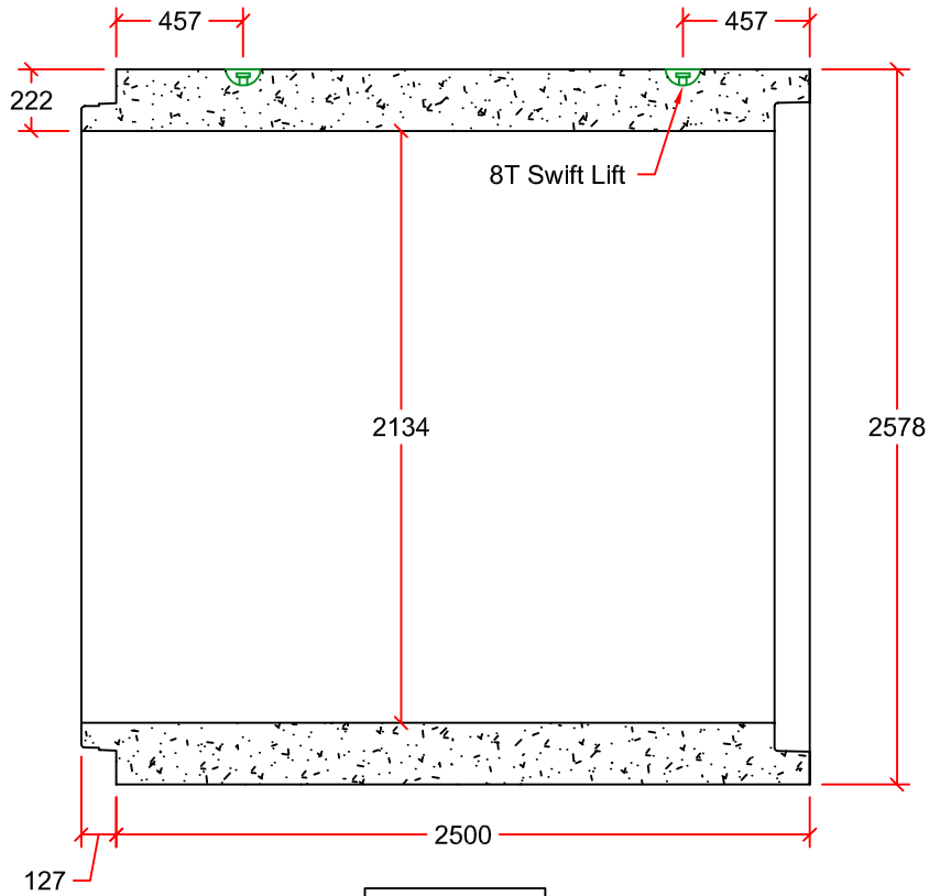
PIPE DETAIL
