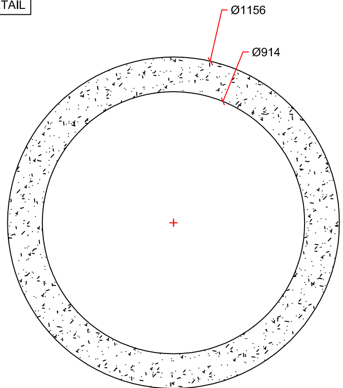
SECTION DETAIL
