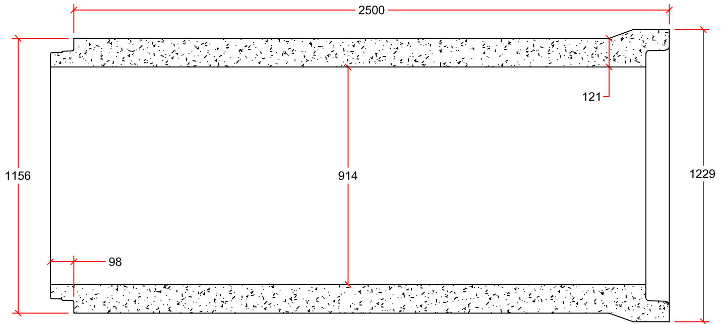
PIPE DETAIL
