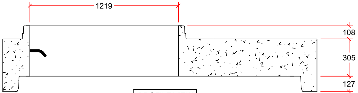
PROFILE VIEW
