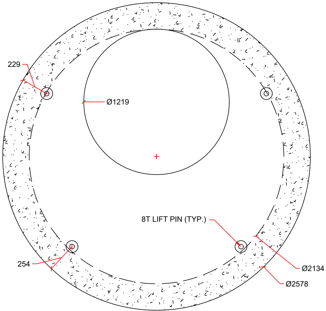
PLAN VIEW
