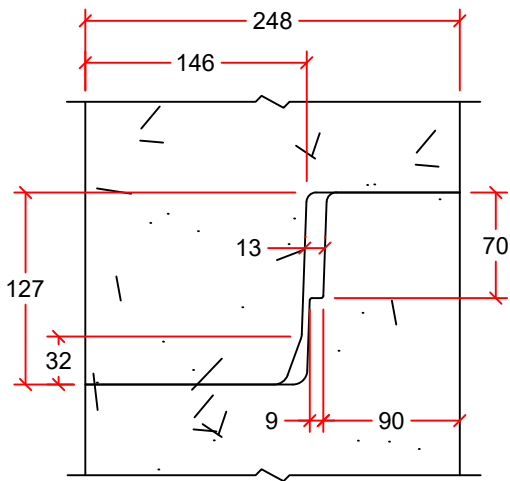
JOINT DETAIL
