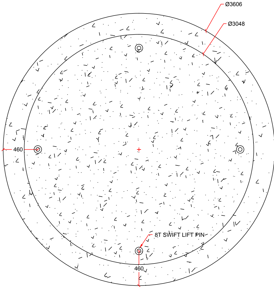
PLAN VIEW
