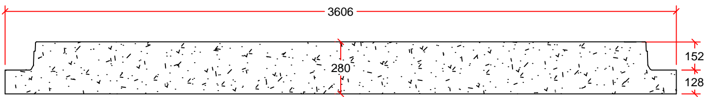
PROFILE VIEW
