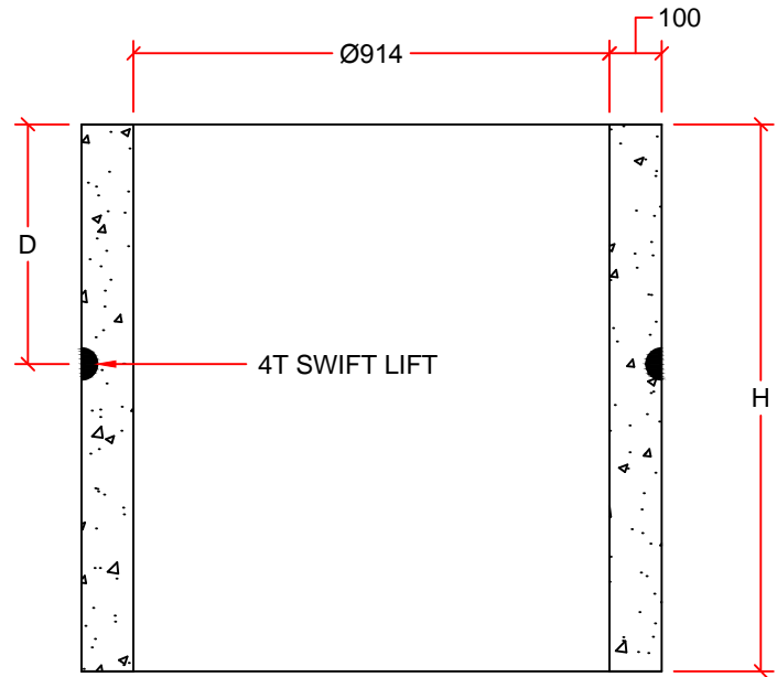
BARRELS AVAILABLE IN 150mm, 300mm, 450mm, 600mm, AND 1050mm HEIGHTS
