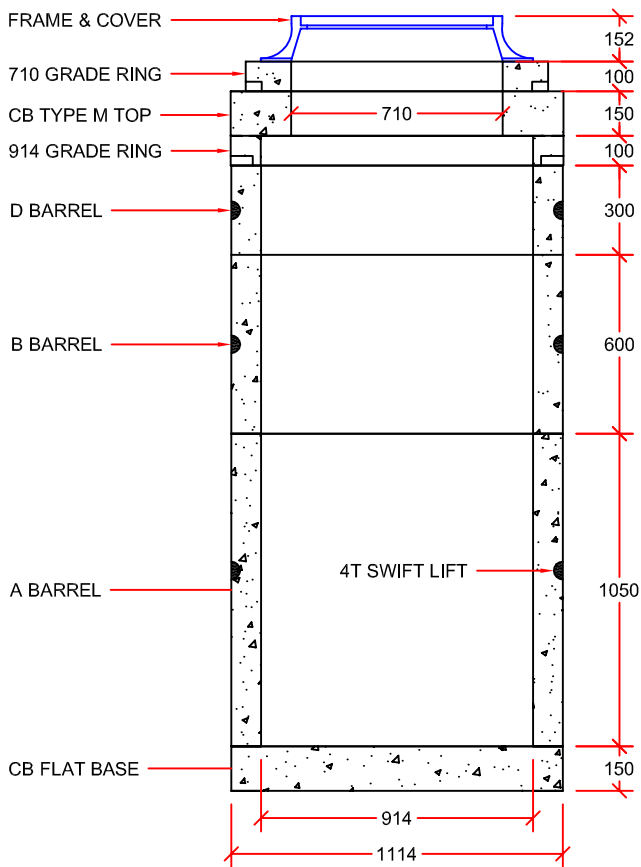
CATCH BASIN W/ SEPARATE BASE
