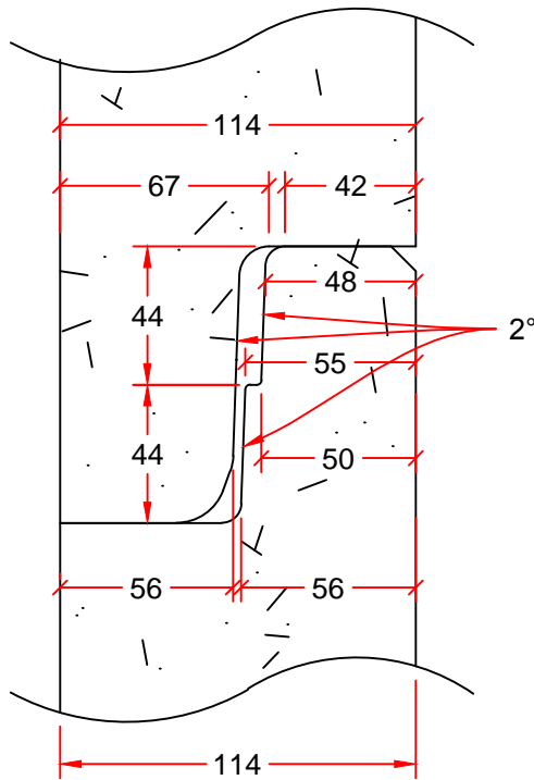
JOINT DETAIL
