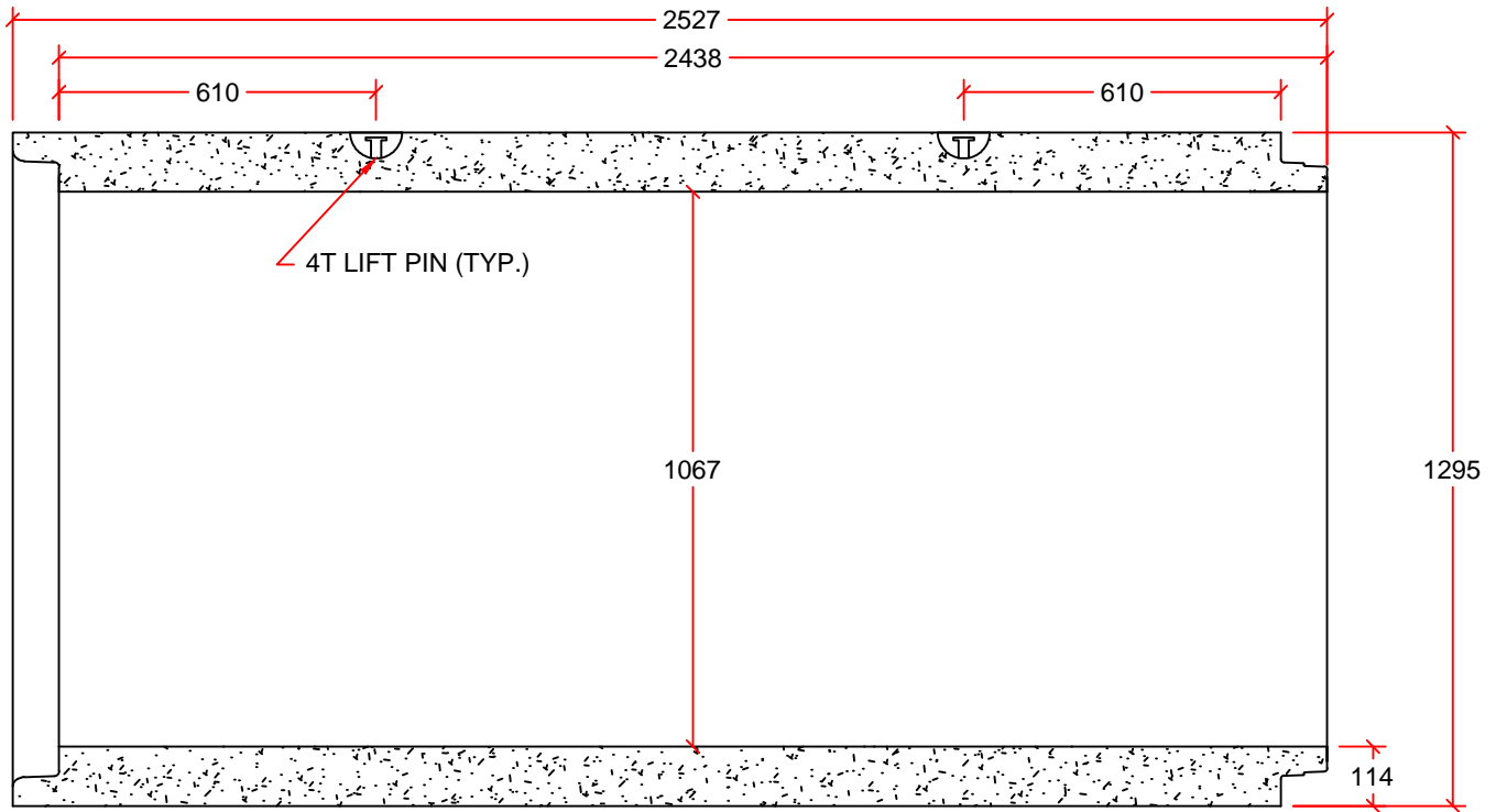
PIPE DETAIL
