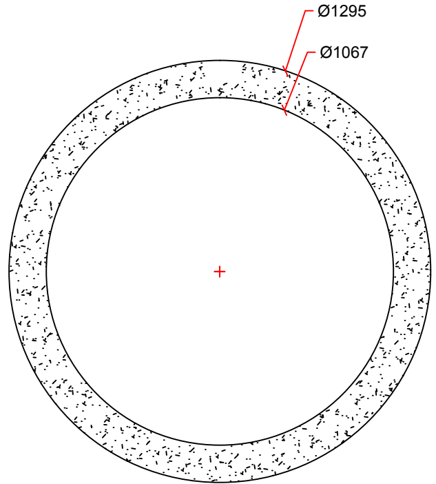
SECTION DETAIL
