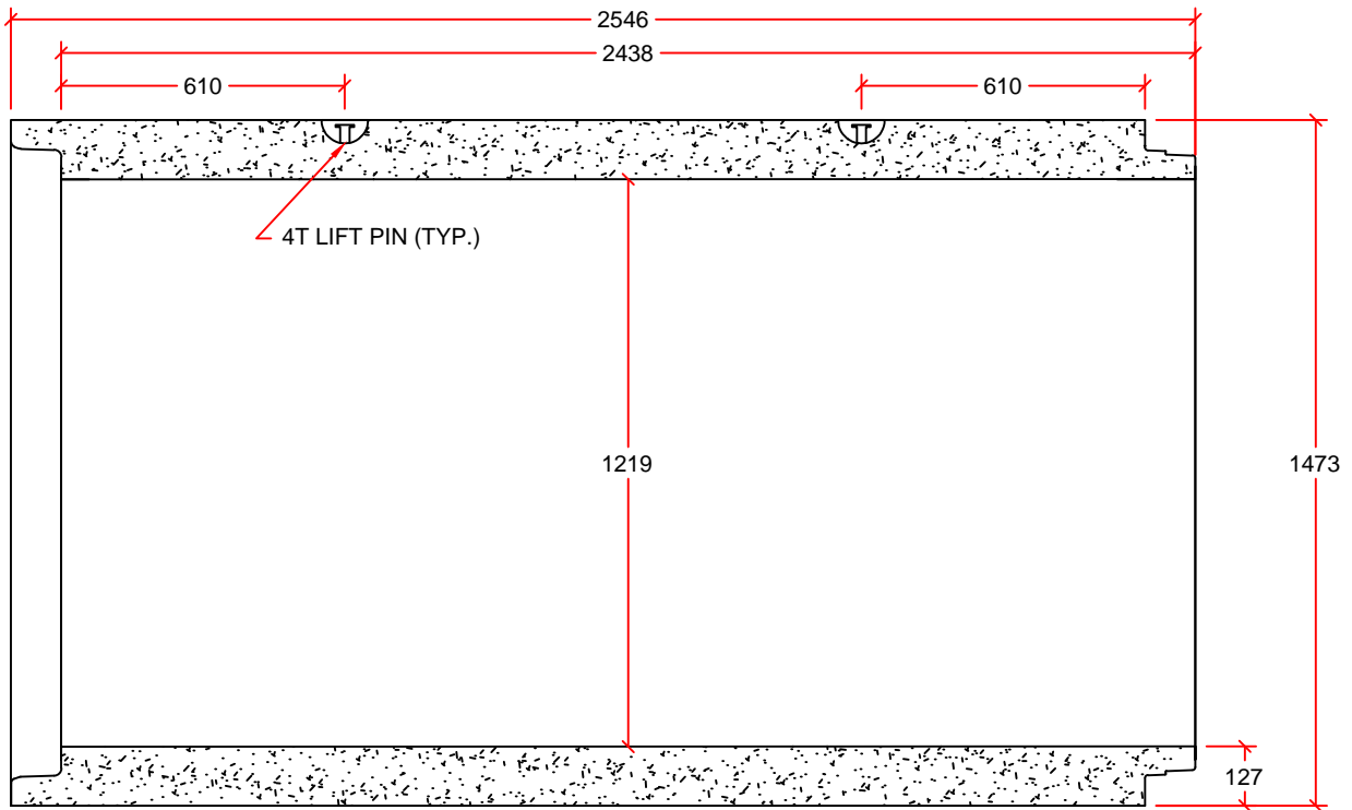
PIPE DETAIL
