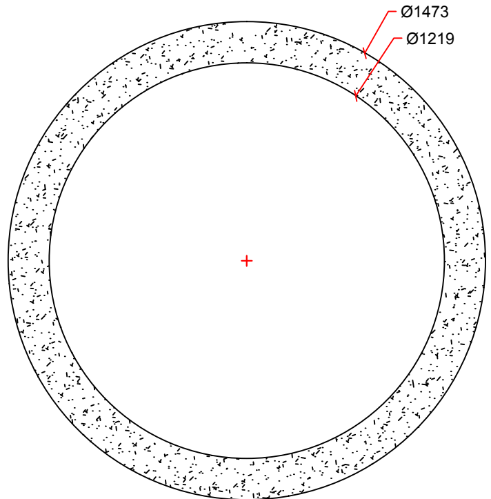
SECTION DETAIL
