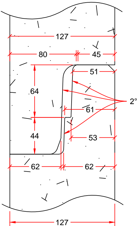
JOINT DETAIL
