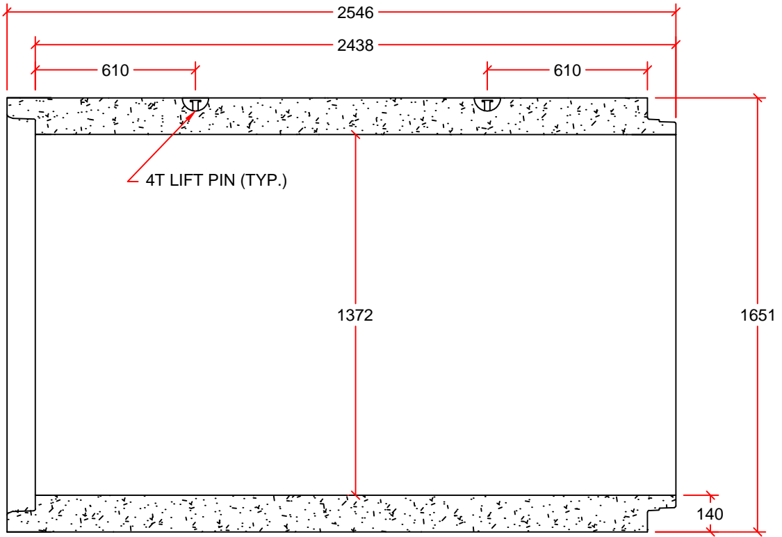
PIPE DETAIL
