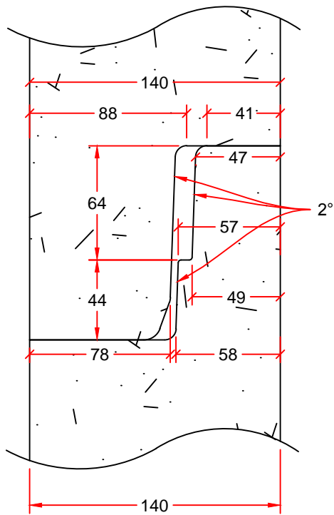
JOINT DETAIL
