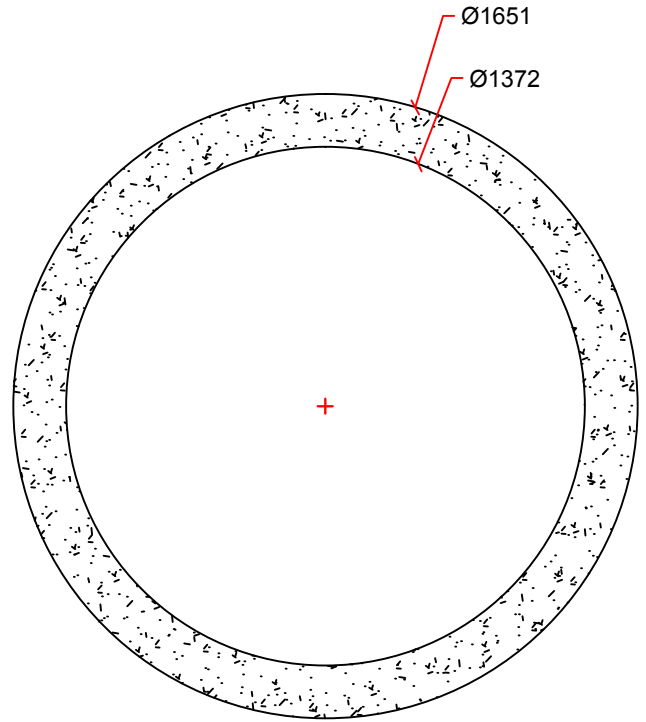
SECTION DETAIL
