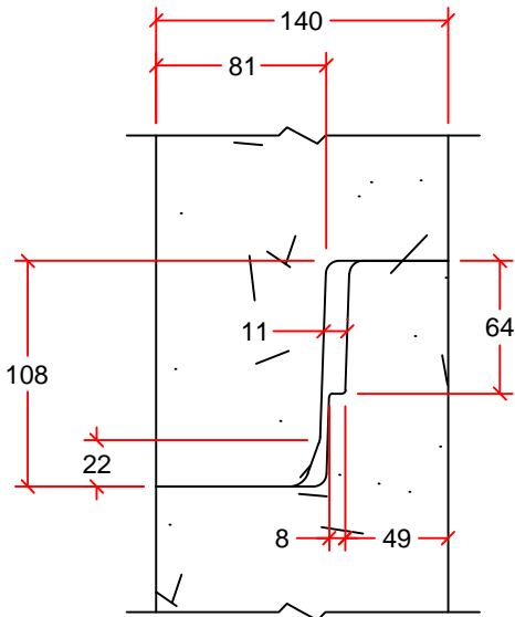
JOINT DETAIL
