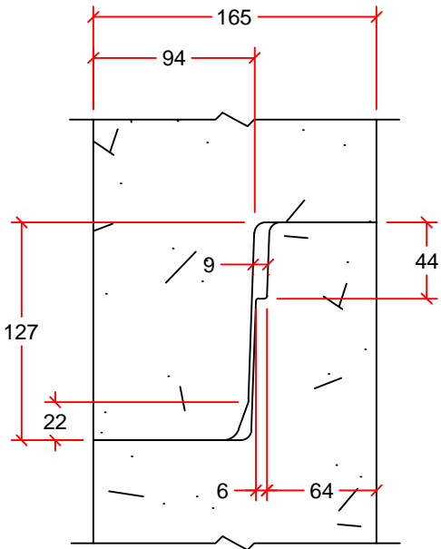
JOINT DETAIL
