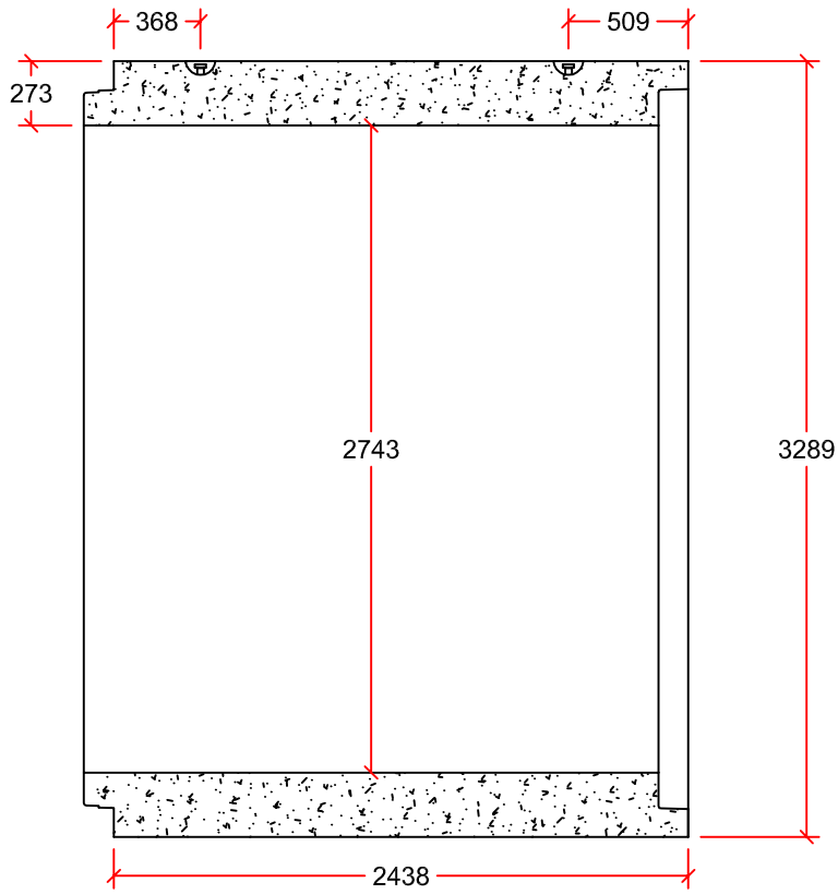
PIPE DETAIL
