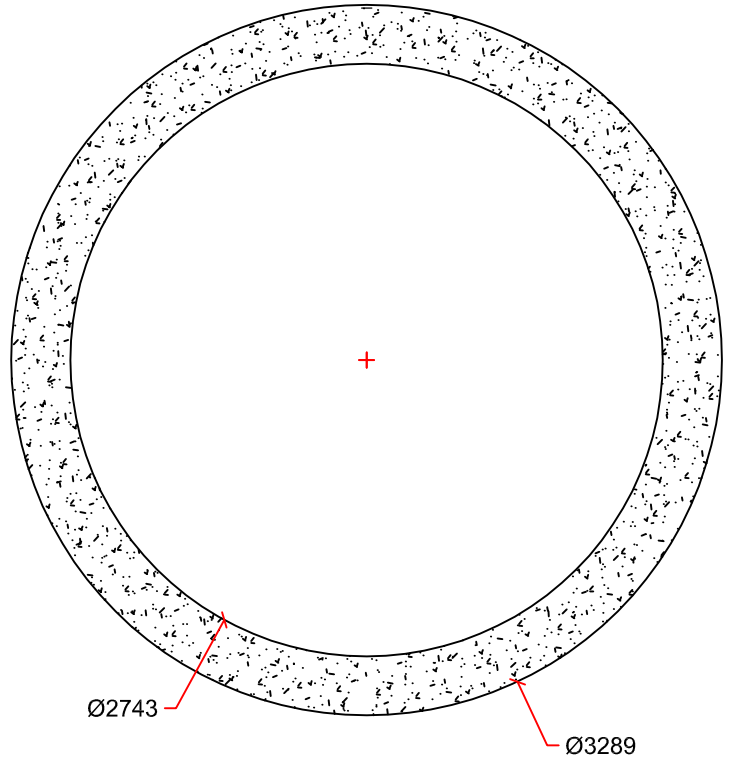
SECTION DETAIL
