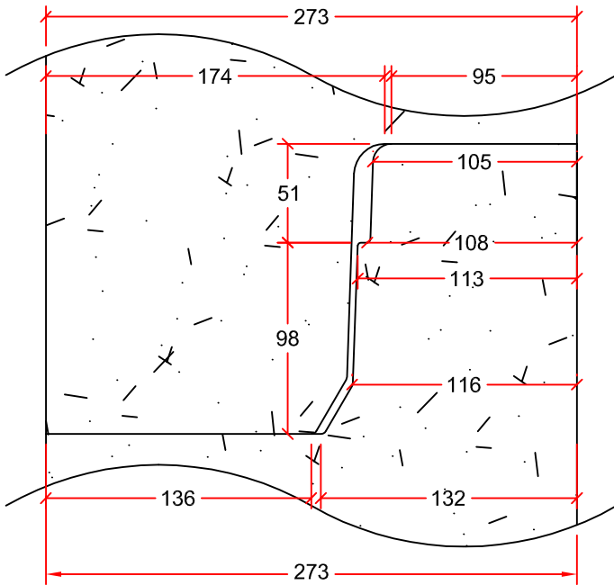
JOINT DETAIL
