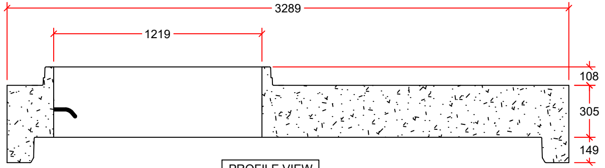
PROFILE VIEW
