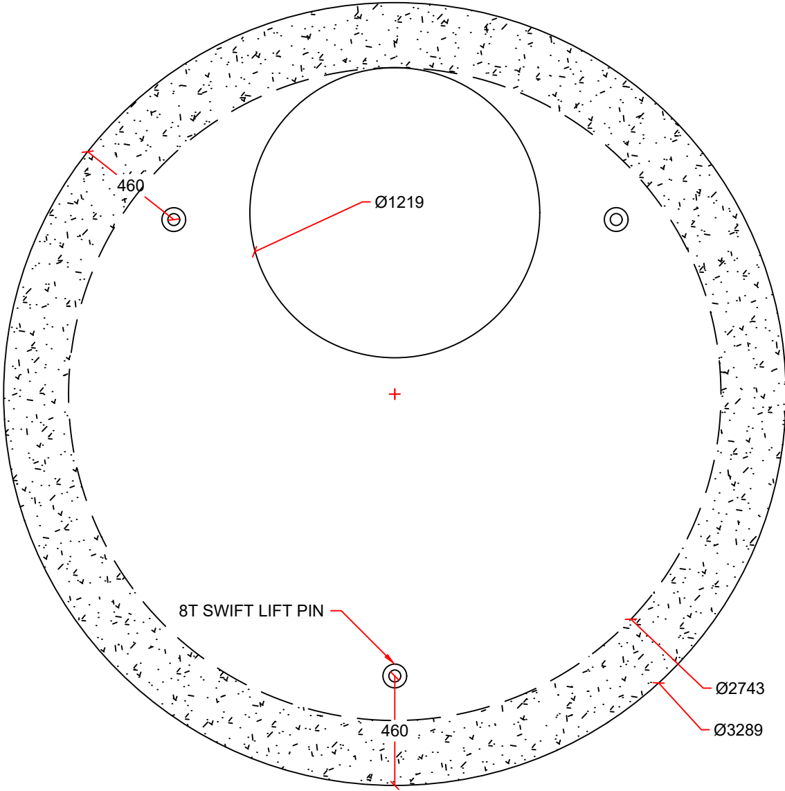
PLAN VIEW
