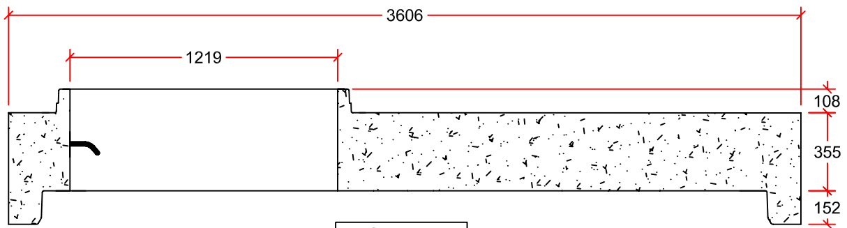
PROFILE VIEW
