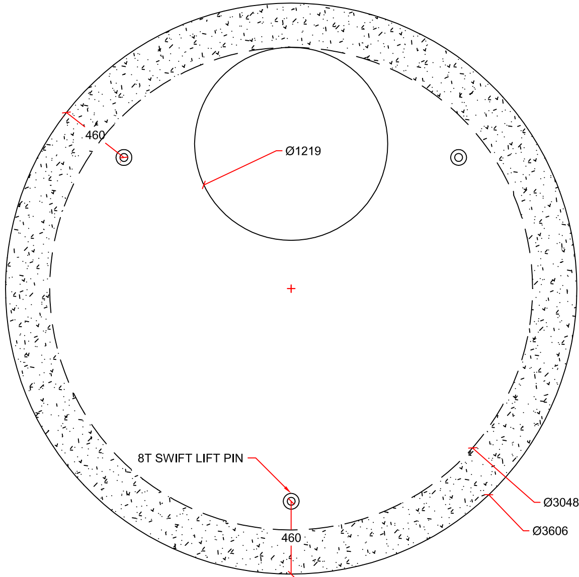
PLAN VIEW
