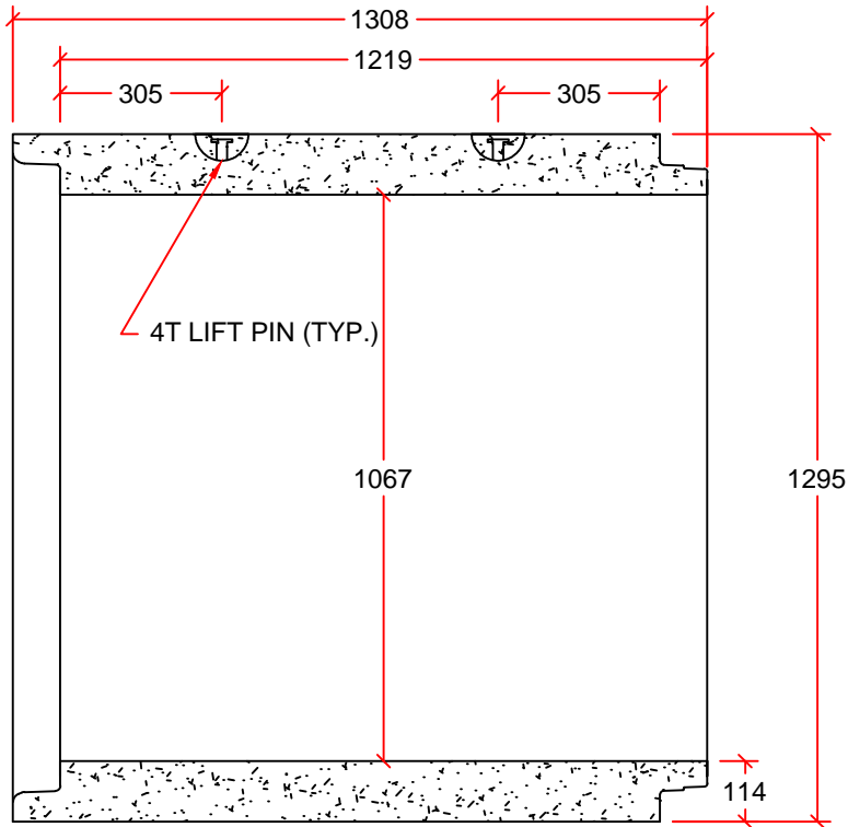
PIPE DETAIL
