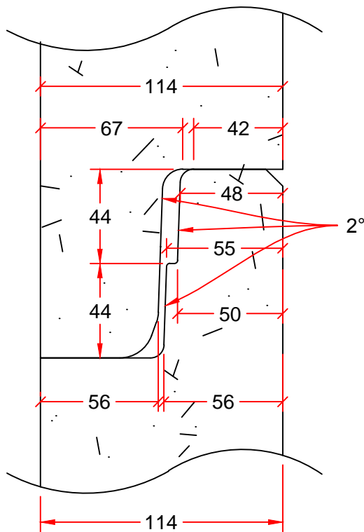
JOINT DETAIL
