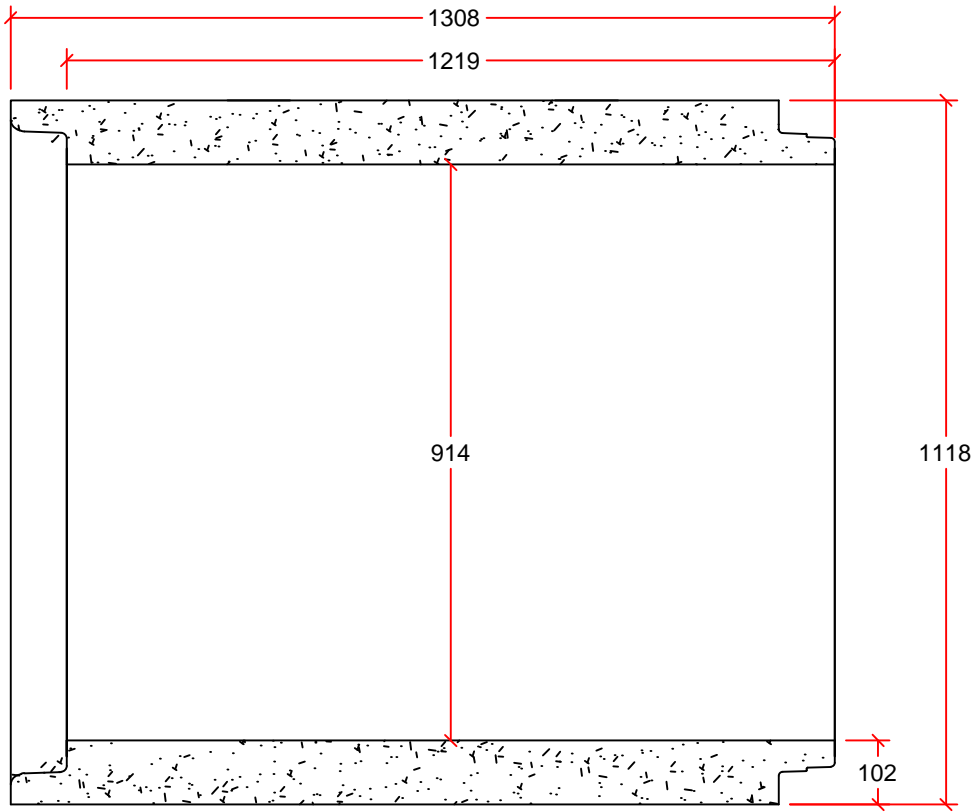
PIPE DETAIL
