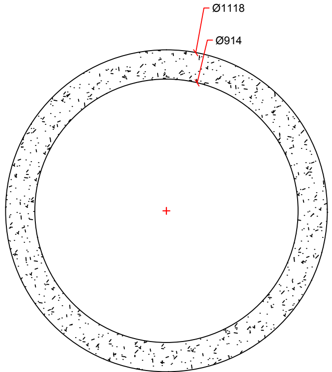
PIPE DETAIL
